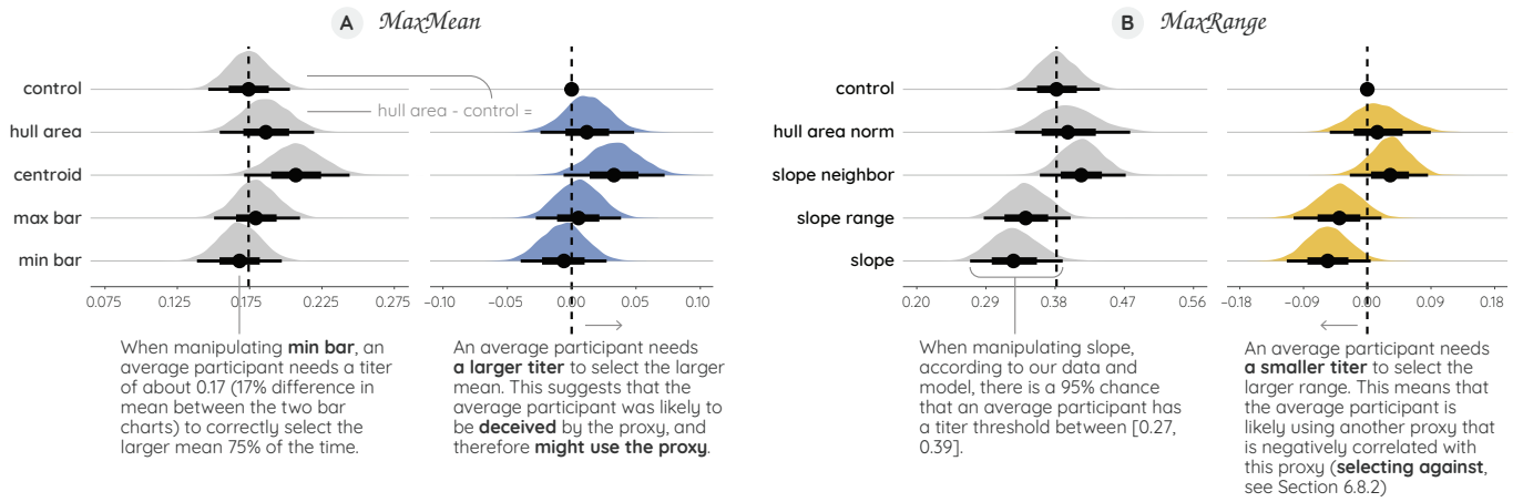
Fig. 4. The effects of manipulating perceptual proxies ( \mathcal{H}_1 ). We show posterior distributions ( \blacktriangle ), 50% and 95% CIs ( \leftarrow\bullet\rightarrow ) of expected titer thresholds, and a comparison with the control condition in both MaxMean and MaxRange tasks.
